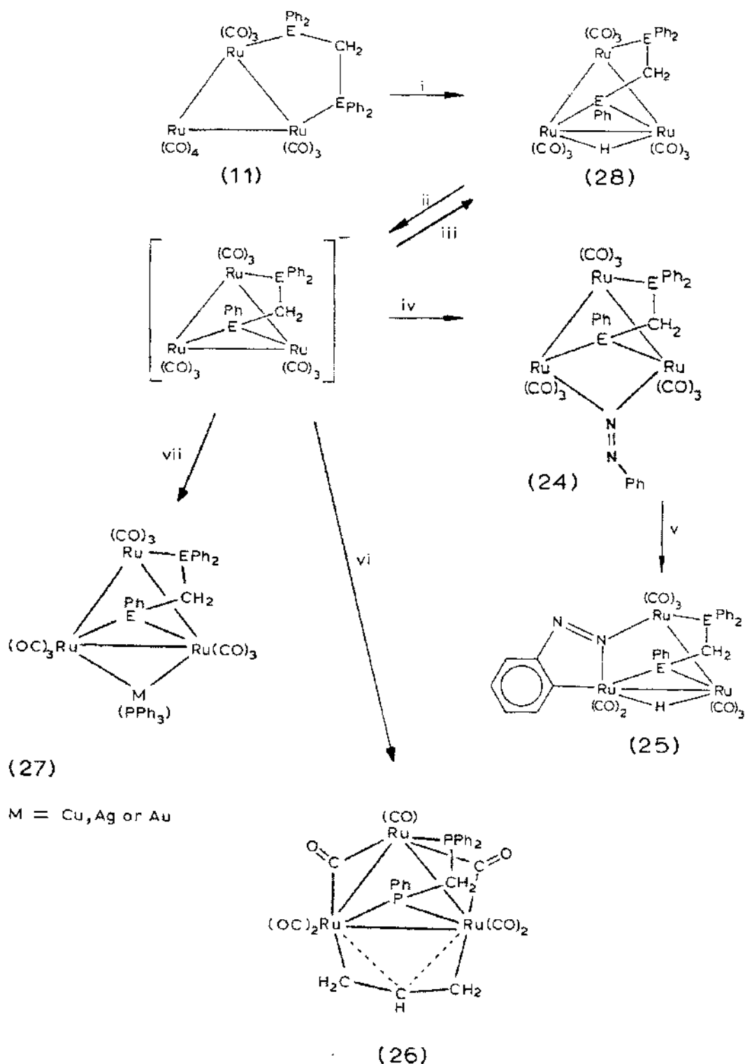
Scheme 6. Some chemistry of \text{Ru}_3(\mu\text{-H})(\mu_3\text{-EPhCH}_2\text{EPh}_2)(\text{CO})_9 . Reagents: (i) \text{H}_2 (20 atm, 80^\circ\text{C} , 20 h); (ii) \text{K}[\text{BHBu}_3] ; (iii) \text{H}^+ ; (iv) [\text{PhN}_2]\text{PF}_6 ; (v) 80^\circ , 1 h; (vi) \text{CH}_2=\text{CHCH}_2\text{Cl} ( \text{E} = \text{P} ); (vii) \text{MCl}(\text{PPh}_3) ( \text{E} = \text{P} , \text{M} = \text{Cu, Ag, Au} ; \text{E} = \text{As} , \text{M} = \text{Au} ).
