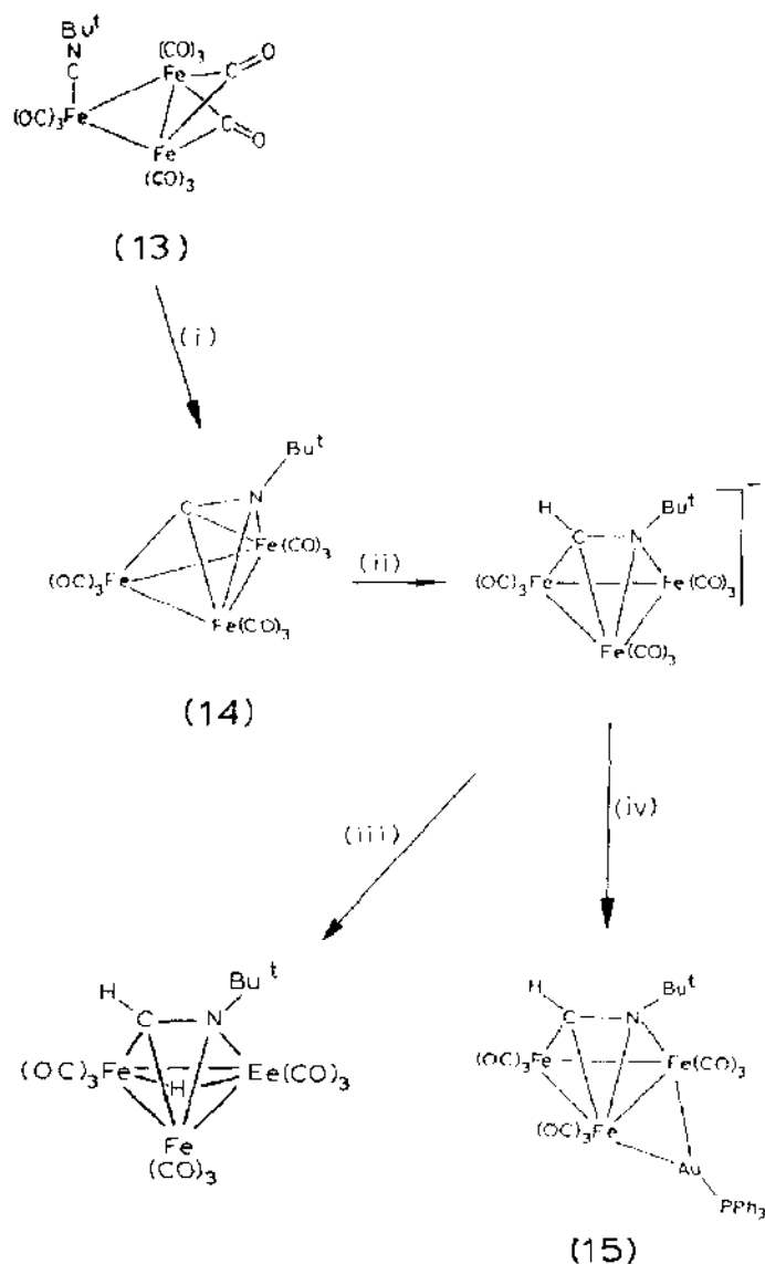
Scheme 4. Some chemistry of \text{Fe}_3(\mu\text{-CO})_2(\text{CO})_9(\text{CNBu}^t) (13). Reagents: (i) Heat at 120^\circ\text{C} ; (ii) \text{K}[\text{HBBu}_3] ; (iii) \text{HPF}_6 ; (iv) \text{AuCl}(\text{PPh}_3) .
